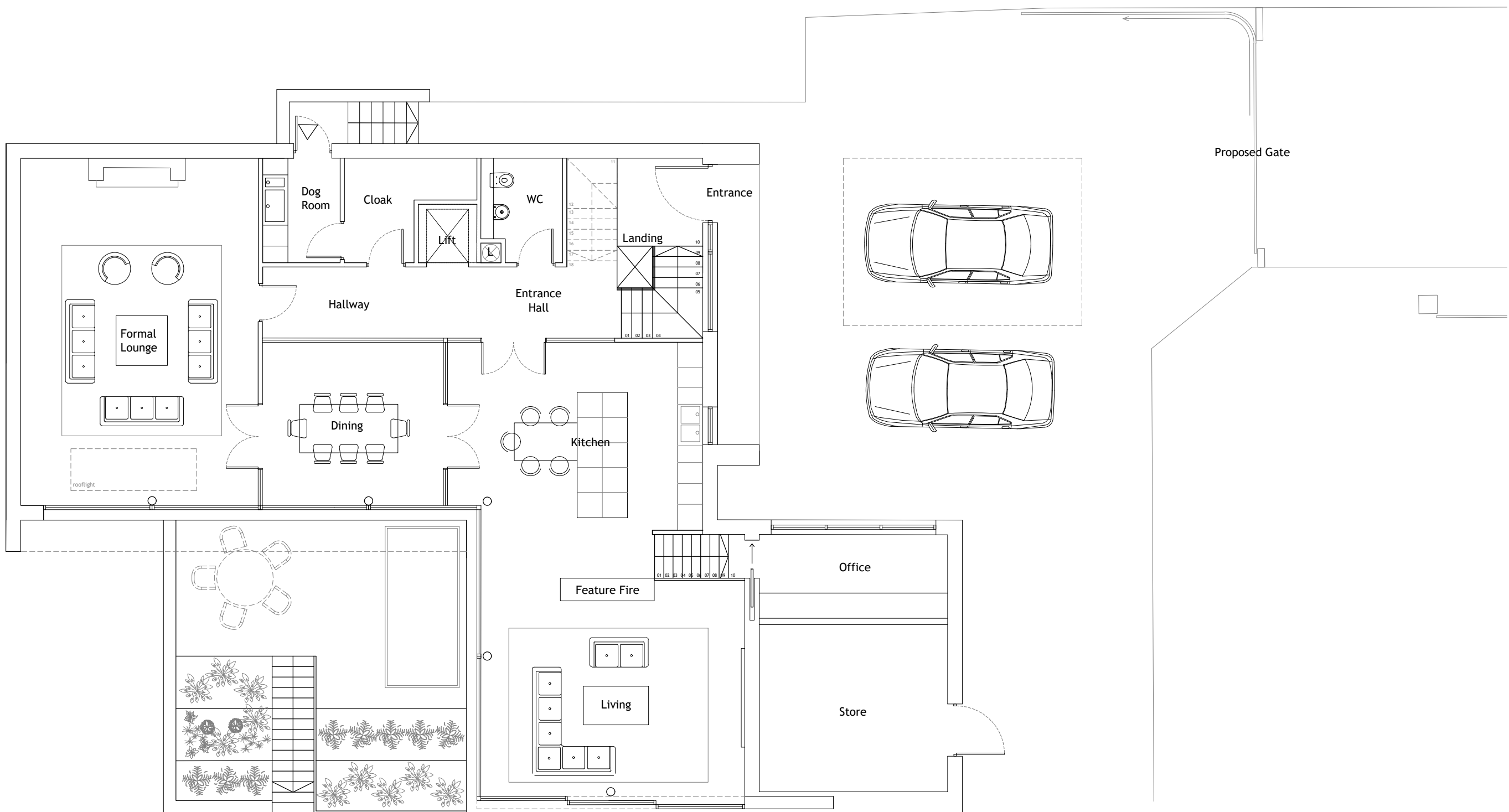
Ground Floor Plan 208m2 / 2239 sqft
