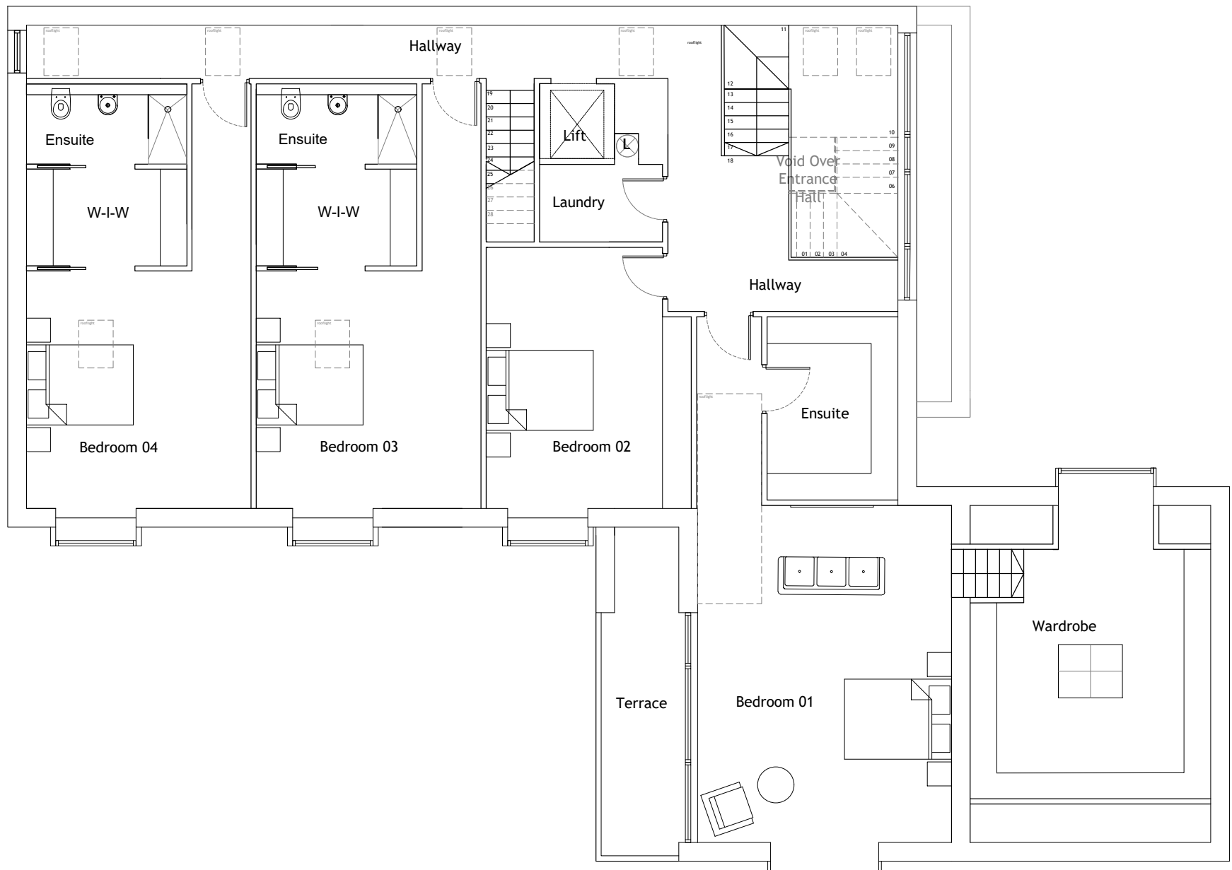
First Floor Plan 190.4m2 / 2049.4 sqft
